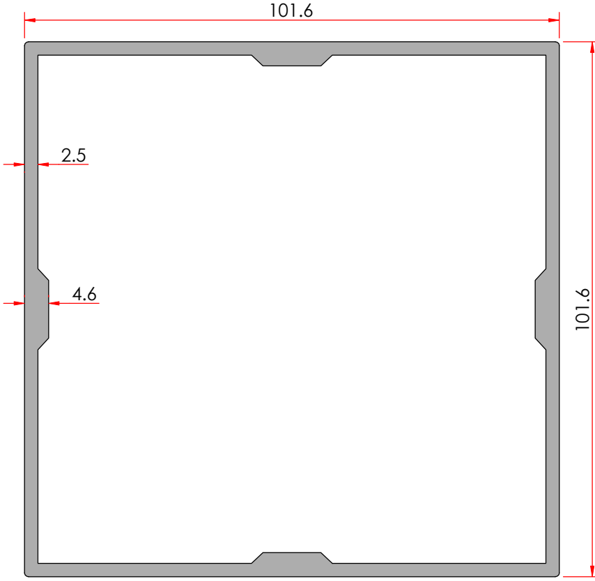
Düsey Yatay Profili Mullion Transom Profile
