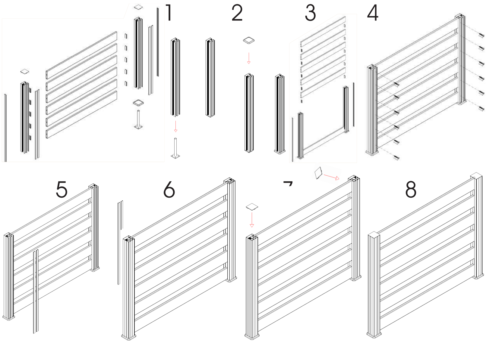
Vertical GoldFence Assembly Drawing
